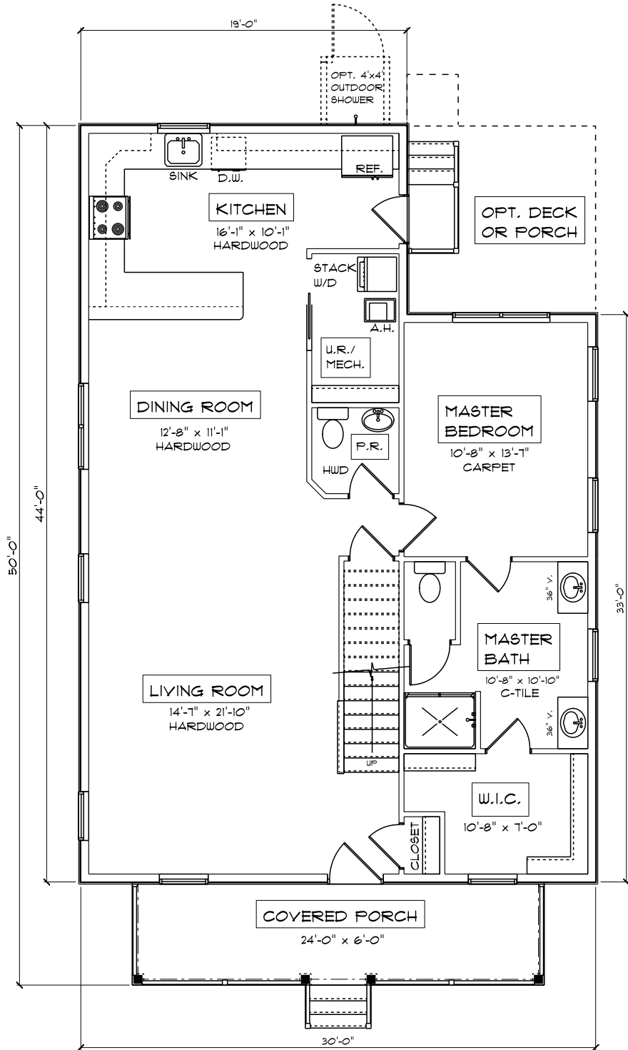
1ST FLOOR PLAN 9' CEILINGS, 1,155 SQFT.
