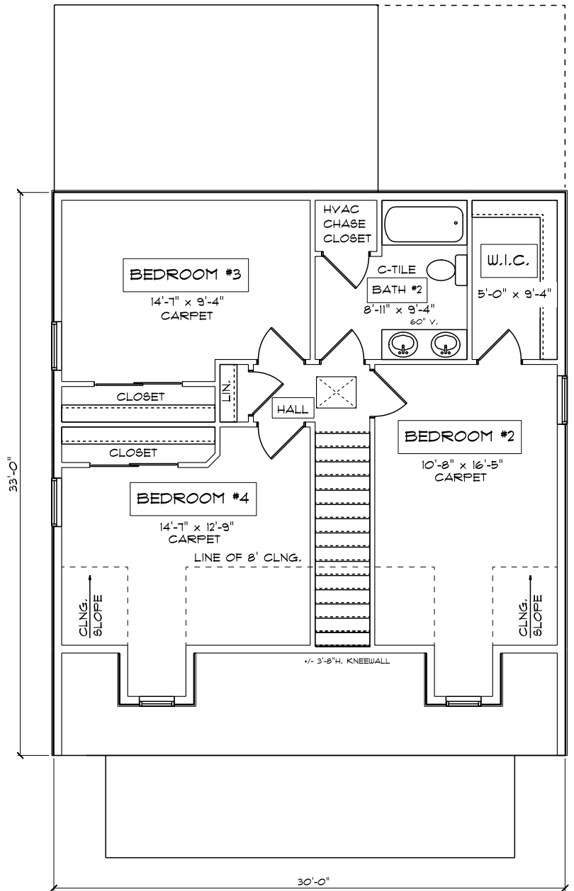
2ND FLOOR PLAN 8' CEILINGS, 795 SQFT.
